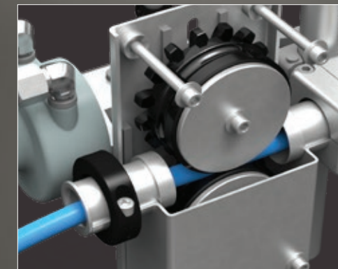
ACCOMMODATES SEVERAL HOSE SIZES Designed to work with 4/4, 5/4, and 6/4 hoses.
