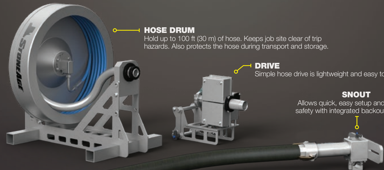
ACCOMMODATES SEVERAL HOSE SIZES Designed to work with 4/4, 5/4, and 6/4 hoses.
