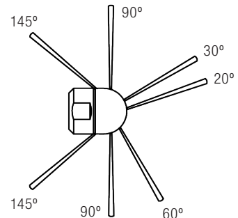
UNIVERSAL 7 Ports: 1 @ 20° 1 @ 30° 1 @ 60° 2 @ 90° 2 @ 145°
